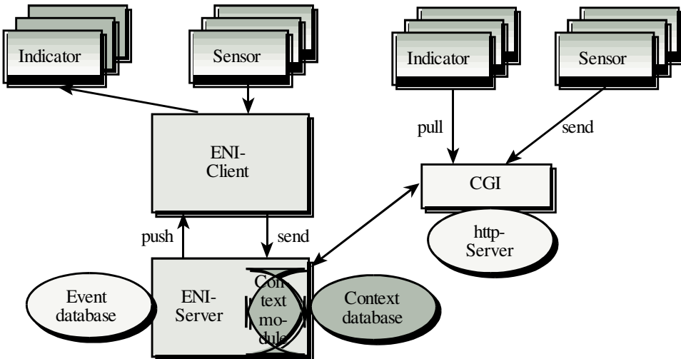
Figure 2. The ENI architecture.
