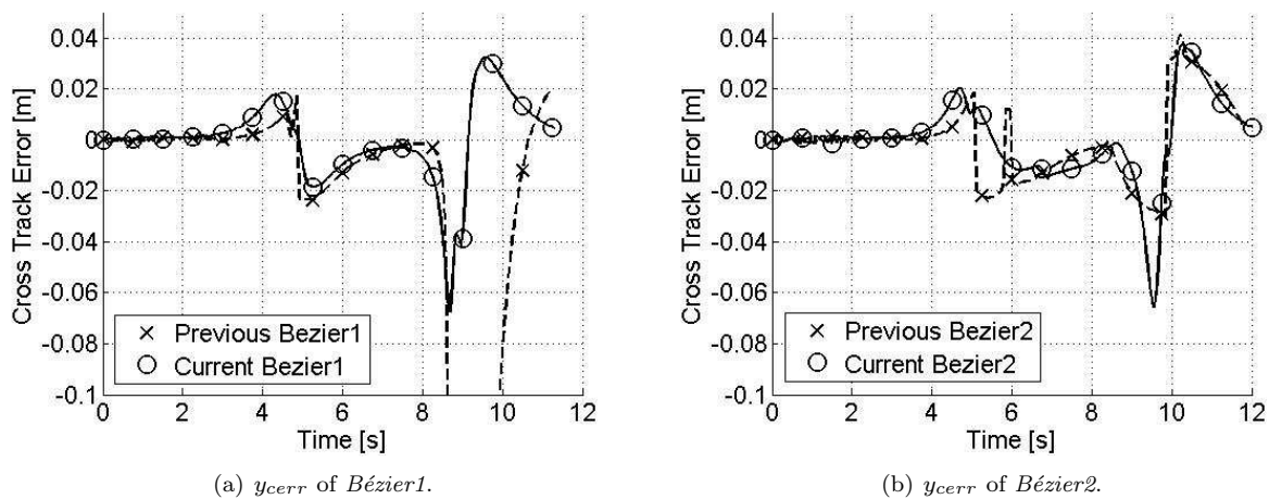
Figure 11: The cross track error y_{cerr} by previous method of [2] (x) and by current method (o). The results of Bézier1 is at left, that of Bézier2 is at right.
