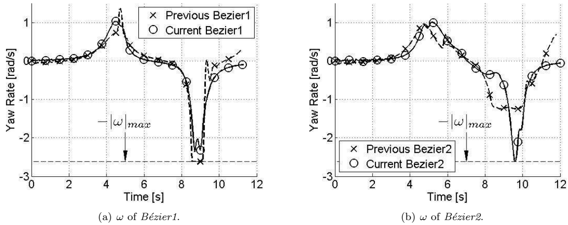
Figure 10: The steering control \omega by previous method of [2] (x) and by current method (o). The results of Bézier1 is at left, that of Bézier2 is at right.
