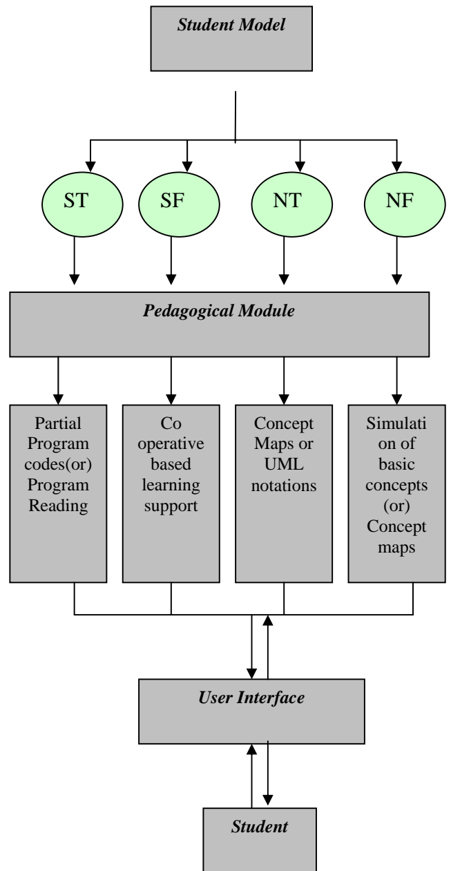
Fig. 2 Proposed framework for visualization
