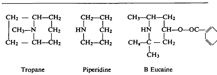
FIG. 3 Importance of ring system.
