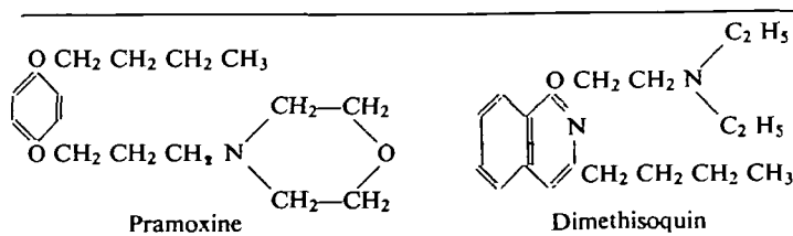
FIG. 10 Amino alkyl ethers.
