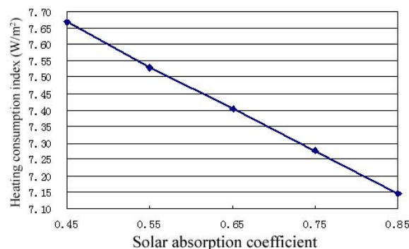
Fig. 4 Solar absorption coefficient vs heating consumption index
