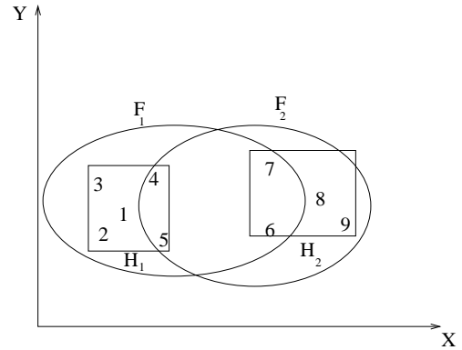
Figure 16. Fuzzy clusters.
