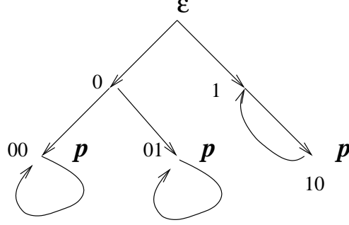
FIGURE 1. A structure of size 6
