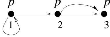
FIGURE 3. Another structure with 3 elements
