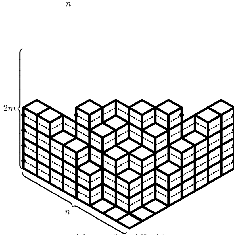
A lozenge tiling of H_{8,4}^-(2)
