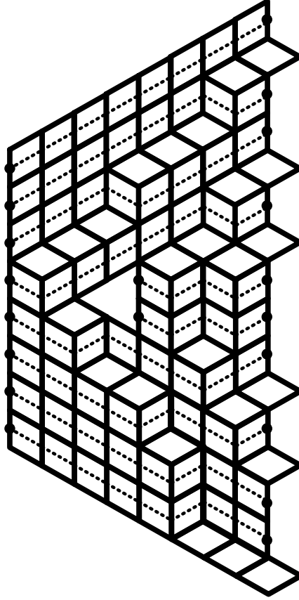
A lozenge tiling of the region F_{8,4}(2) ; the right boundary is free. The dotted lines mark paths of lozenges. They determine the tiling uniquely.
