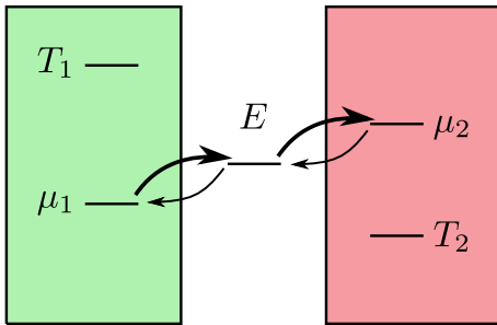
Figure 8. In a thermoelectric device, simplified here as a quantum dot with a single relevant energy level E , electrons are transported on average from a hot reservoir with \mu_1 and T_1 to a cold reservoir with \mu_2 = \mu_1 + \Delta\mu > \mu_1 and T_2 = T_1 - \Delta T using heat from the hot reservoir.
