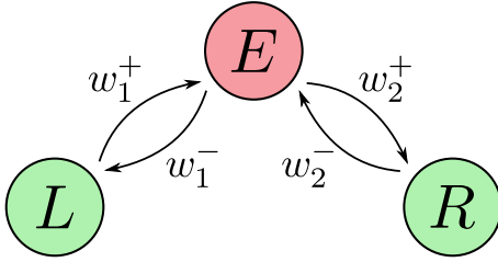
Figure 9. Common three-state diagram for the simplified BL ratchet (Fig. 7) and the thermo-electric device (Fig. 8). For the BL-ratchet L and R refer to the particle sitting in the minimum and E corresponds to the particle being on the barrier top. For the electronic device, L and R refer to the electron being in the left or right reservoir. E corresponds to the electron sitting on the quantum dot. In both cases, the state R should be identified with L after the electron or particle has been transported from left to right thus completing the cycle. The log-ratio of the transition rates is given in Tab. 2.
