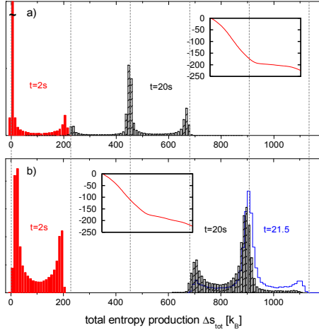
Figure 2. Distribution of entropy production p(\Delta s^{\text{tot}}) for a colloidal particle driven along a periodic potential for two different values of external force f [144]. The insets show the total potential v(x) - fx . The different histograms refer to different trajectory lengths.
