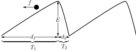
Figure 7. In a BL ratchet, a particle preferentially climbs a potential barrier with height E over a distance d_1 while in contact with a heat bath at T_1 . It slides down a distance d_2 on the cold side with T_2 = T_1 - \Delta T . This temperature-difference driven motion to the right persists for a small enough force f < 0 pulling to the left.
