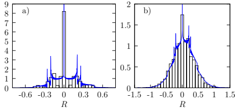
Figure 5. Probability distribution for the “work” (137), denoted here R , in a driven two-level system for two different lengths of trajectories. The histogram are experimental data, the full curve a theoretical calculation, for more details, see [88].
