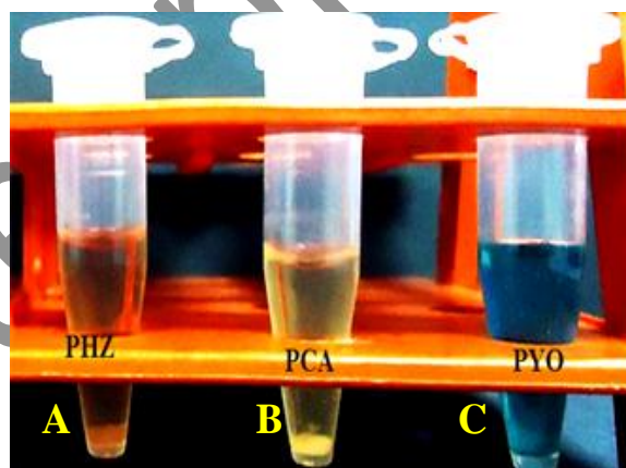
Fig. 2: Different colour indicates different antibiotics in benzene and chloroform fraction during extraction phase. A= Extract of phenazine (bright orange colour), B= Extract of PCA (lemon yellow colour) and C= Extract of pyocyanin (blue colour)
