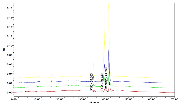
Fig. 3: Chromatographic separation of phenazine (PHZ), phenazine-1-carboxylic acid (PCA) and pyocyanin (PYO) from standard mixture at 1000 µg/mL concentration with various retention times at 250 nm wave length
