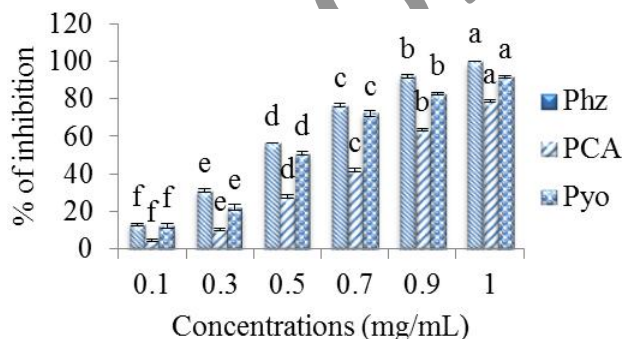
Fig. 8: Percent growth inhibition of Ganoderma boninense at different concentrations of phenazine, PCA and pyocyanin after 7 days of treatment. Values followed by the same letter are not significantly different according to LSD test at P \leq 0.05 level. Each value is the mean of 3 replications. Vertical bars represent standard error
