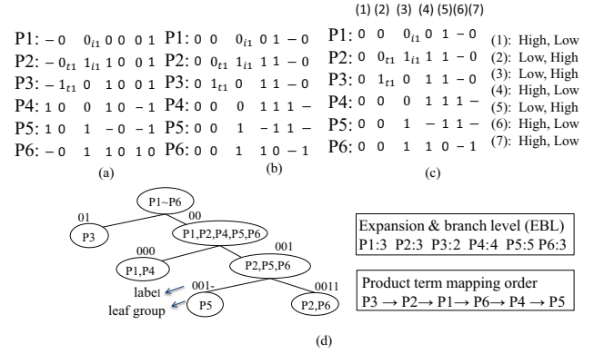
Fig. 6. An example. (a)(b) Variable reordering. (c) Architecture determination. (d) Grouping tree construction and EBL estimation.
