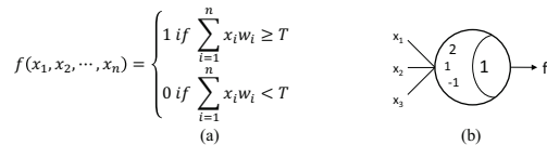
Fig. 3. (a) The definition of an LTG. (b) An LTG implementing the function f = x_1 + x_2x_3 .
