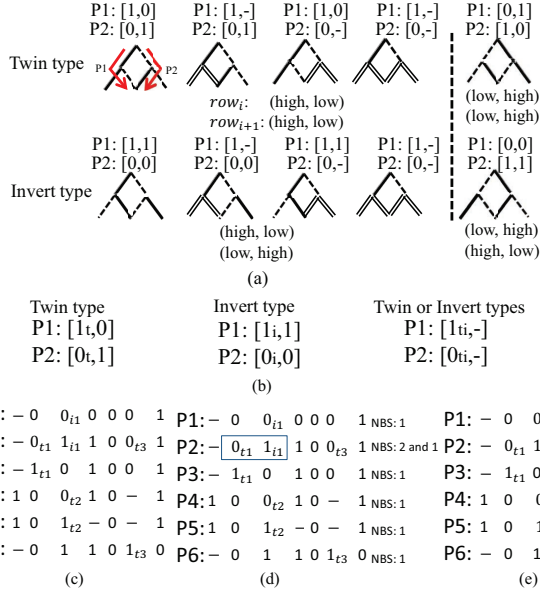
Fig. 5. (a) The types of Branch-then-Shares. (b) Notations of Branch-then-Shares. (c)~(e) The demonstration of collecting Branch-then-Shares.
