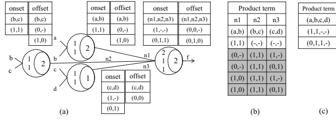
Fig. 4. An example for demonstrating the computation of product terms from a threshold network.
