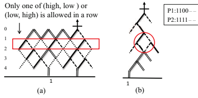
Fig. 2. (a) The fabric constraint. (b) 2-bit Branch-then-Share.
