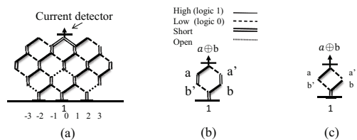
Fig. 1. (a) An SET array fabric. (b) An example of a \oplus b . (c) A simplified diamond-shaped network of a \oplus b [3].
