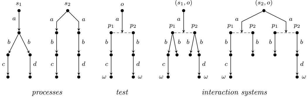
Figure 8: NPLTS models equated by \sim_{\text{Te,find}} and distinguished by \sim_{\text{PTe-}\cup}/\sim_{\text{PTe-}\exists}
