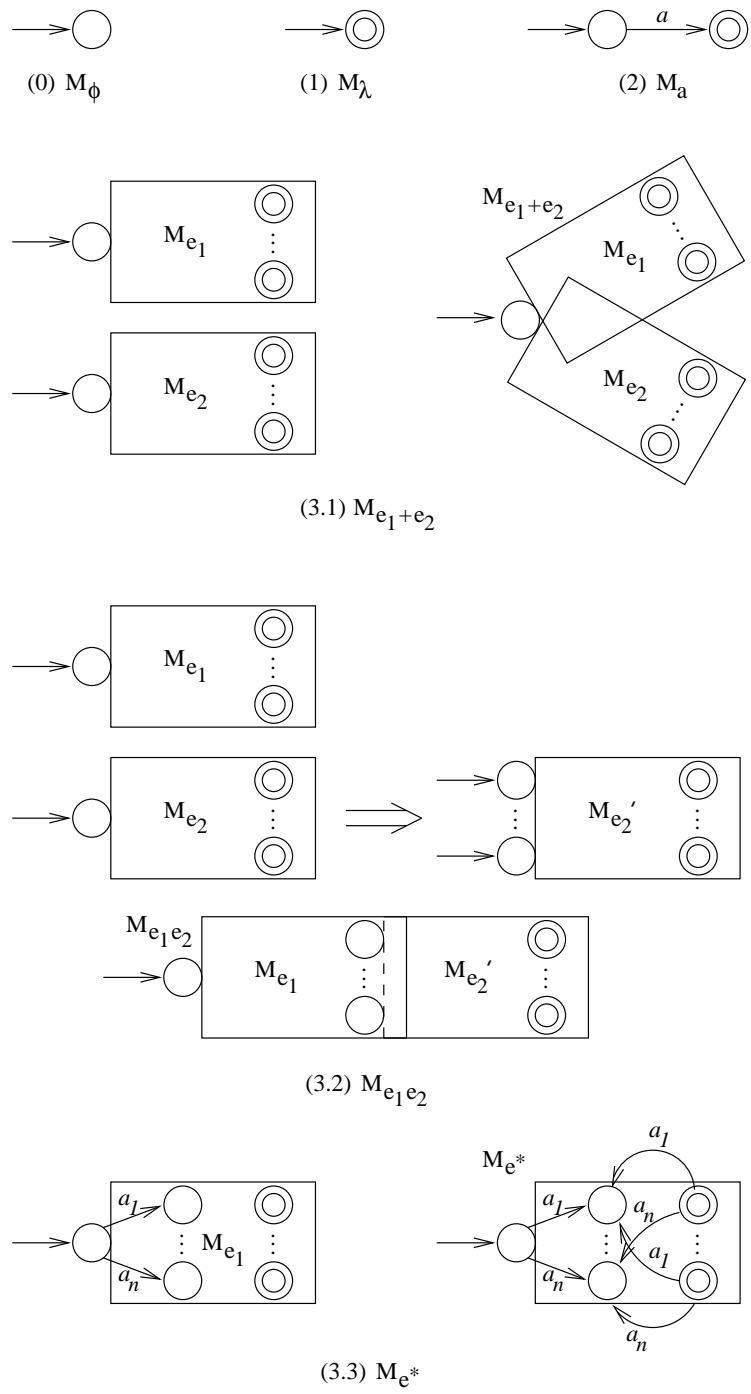
Figure 11: A Regular Expression to an NFA without \lambda -Transitions
