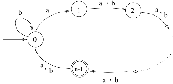
Figure 17: An n -state DFA A_n : The language (L(A_n))^* requires 2^{n-1} + 2^{n-2} states
