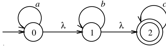
Figure 5: A \lambda -NFA A_3
