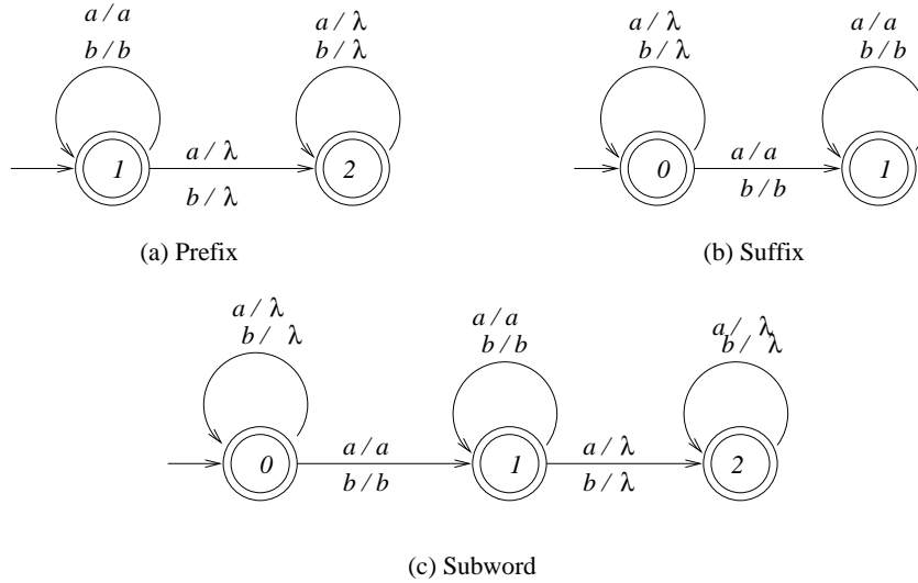
Figure 13: Finite transducers realizing the prefix, suffix, and subword operations
