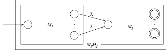
(b) Catenation
