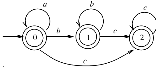
Figure 6: An NFA A'_3
