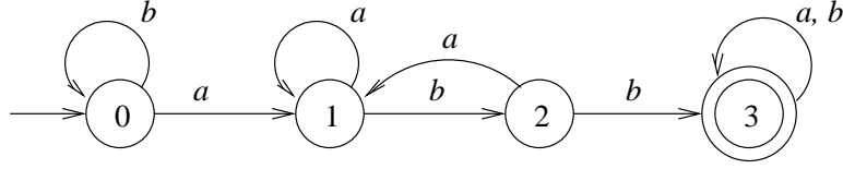
Figure 2: A deterministic finite automaton A_1
