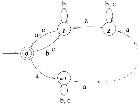
Figure 18: An n -state DFA such that L(A)^R requires 2^n states
