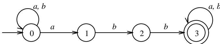
Figure 3: A nondeterministic finite automaton A_2
