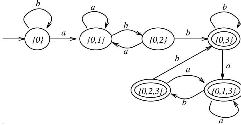
Figure 4: A DFA A_6 equivalent to NFA A_2
