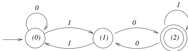
Figure 1: The states and transition rules of A_0
