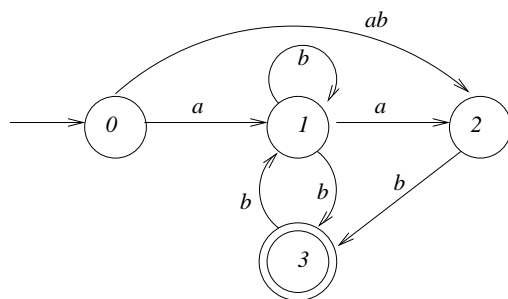
(a) Given EFA
