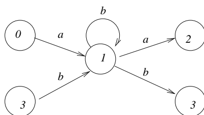
(b) Working sheet for deleting State 1
