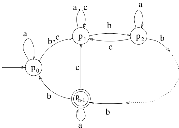
Figure 16: DFA B
