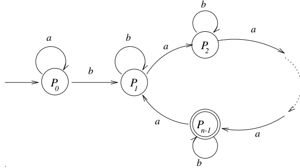
Figure 14: DFA B
