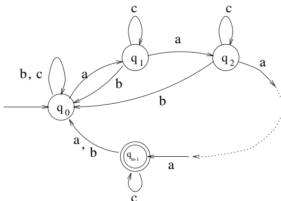
Figure 15: DFA A
