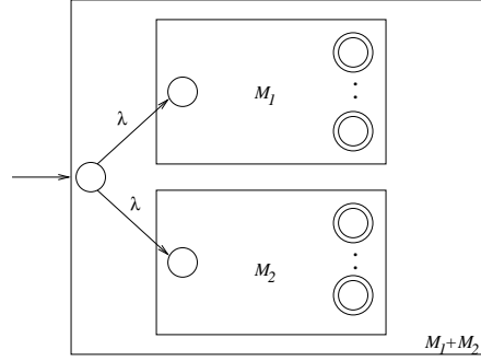
(a) Union
