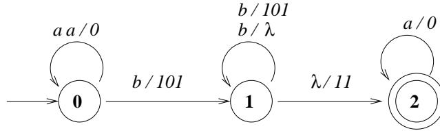
Figure 9: A finite transducer T
