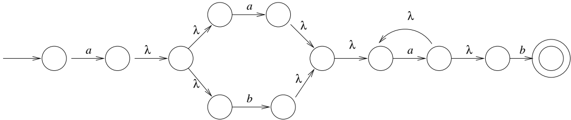
Figure 10: A \lambda -NFA constructed for a(a + b)a^*b
