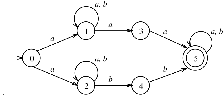
Figure 8: An NFA A_4
