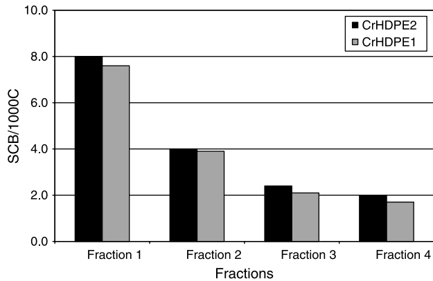
Fig. 3. The total amount of short chain branches (SCB/1000C atoms) per preparative TREF fraction determined by ^1\text{H} NMR.
