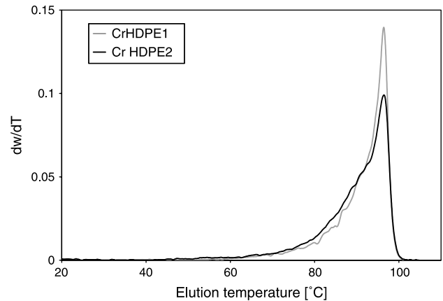
Fig. 2. TREF chromatographs of CrHDPE1 and Cr HDPE2.
