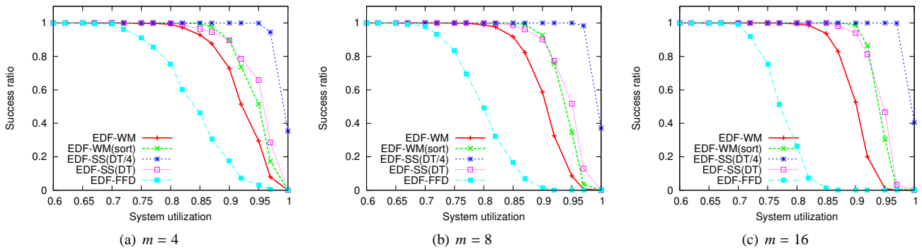
Figure 8. Guaranteed schedulability: (u_{min}, u_{max}) = (0.5, 1.0) .
