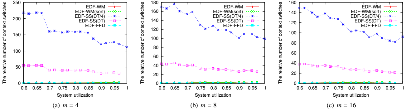
Figure 11. The worst-case number of context switches relative to EDF-FFD: (u_{min}, u_{max}) = (0.5, 1.0) .
