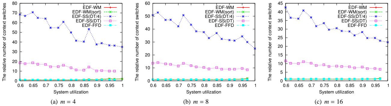
Figure 12. The worst-case number of context switches relative to EDF-FFD: (u_{min}, u_{max}) = (0.1, 0.5) .
