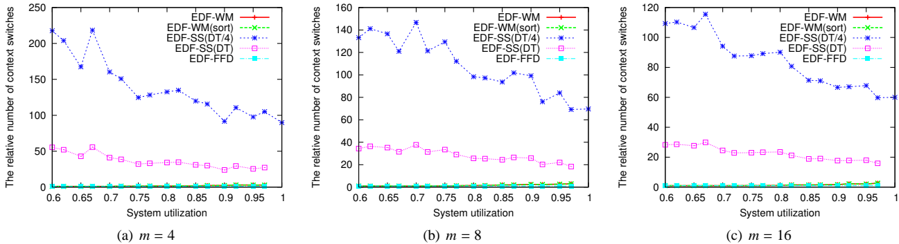
Figure 10. The worst-case number of context switches relative to EDF-FFD: (u_{min}, u_{max}) = (0.1, 1.0) .
