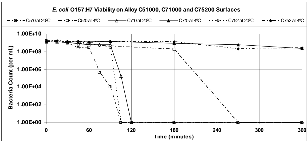
Figure 3: E. coli O157:H7 Viability on the Surfaces of Alloys UNS C51000, C71000 and C75200 at 20°C and 4°C.
