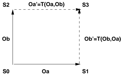
(a) Transformation property 1: O_a \circ O_b' \equiv O_b \circ O_a'
