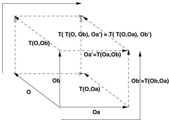
(b) Transformation property 2: T(T(O, Oa), Ob') = T(T(O, Ob), Oa')
