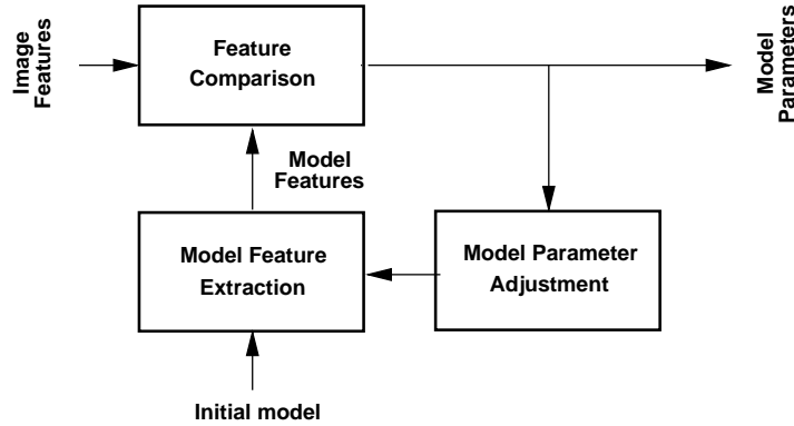
Figure 6: 3D Hand/arm model parameter computation through successive approximation technique.
