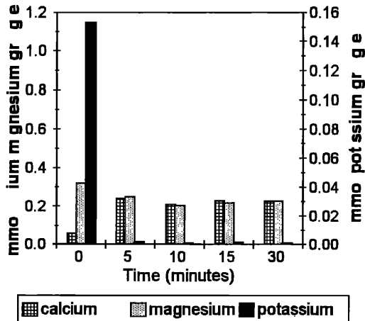
Figure 3. The effect of pH value, temperature, and exposure time to Dead Sea concentrated brine (Mineral Skin Osmoter™) on the biosorption of elements to Dunaliella salina algal biomass. Blank values relate to non-treated algae.
