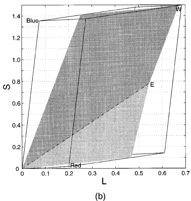
Fig. 2. Parallel projections of the video monitor gamut limits and reduced stimuli surfaces along (a) the L axis as for the protanopic simulation, (b) the M axis as for the deuteranopic simulation, and (c) the S axis as for the tritanopic simulation. The shaded wings in (a) and (b) go toward 475 nm and 575 nm, and the wings in (c) go toward 485 nm and 660 nm.
