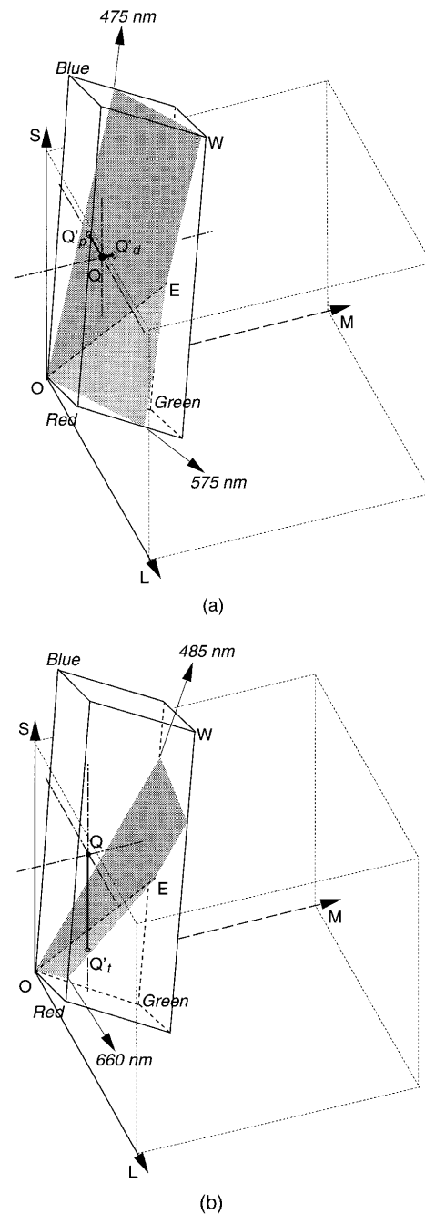
Fig. 1. Geometric representation of the algorithm to simulate dichromatic vision. The axes L , M , and S represent the quantum catch for each of the three classes of cones. The limits of the parallelepiped define the gamut of color stimuli that could be obtained on the video monitor used for the simulation. \mathbf{W} represents the nominal White stimulus obtained with Red, Green, and Blue video channel signals at maximum. \mathbf{E} represents the brightest possible metamer of an equal-energy stimulus on this monitor. The line OE represents the neutral stimuli for dichromats as well as for normal trichromatic observers. (a) The wings from OE toward the 475-nm and 575-nm locations represent the reduced stimuli surface for protanopic and deuteranopic simulation; (b) the wings from OE toward 485 nm and 660 nm represent the reduced stimuli surface for tritanopic simulation. The simulation algorithm consists in replacing the physiologically undetermined component by the corresponding values on the respective reduced stimuli surface. This is illustrated for a given color stimulus \mathbf{Q} , which is replaced by \mathbf{Q}'_p for the protanope, by \mathbf{Q}'_d for the deuteranope, and by \mathbf{Q}'_t for the tritanope.
