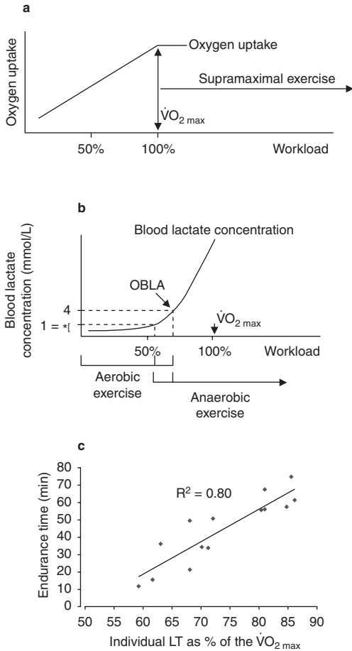
Fig. 4. Terminology used in exercise physiology and its physico-physiological meaning. (a) Relationship between workload and oxygen uptake. Workloads above maximal oxygen uptake ( \dot{V}O_{2max} ) are 'supramaximal workloads'. At these supramaximal workloads, most of the power is produced by type II muscle fibres, which generate their intracellular adenosine triphosphate (ATP; necessary for the cross-bridge interaction), by the glycolytic pathway and breakdown of creatine phosphate. (b) Relationship between workload and blood lactate concentration. The different definitions for the lactate threshold (LT; exceeding 1 mmol/L increase of the baseline) and the onset of blood lactate accumulation (OBLA; 4 mmol/L) are shown. In this graph, aerobic exercise is defined as the workload until the lactate threshold or OBLA has been reached. The anaerobic threshold is the workload beyond lactate threshold and OBLA. During aerobic exercise, muscle power is produced predominantly by type I muscle fibres, which generate most of their ATP via the aerobic pathway. The aerobic exercise ends at about 50% \dot{V}O_{2max} in untrained subjects and at more than 80% \dot{V}O_{2max} in very well trained subjects. (c) Relationship between LT and endurance time. The LT was defined as the workload at which the blood lactate concentration exceeded the 1 mmol/L of baseline. The endurance time was estimated during a workload at 88% \dot{V}O_{2max} in 14 volunteers (data obtained from Coyle et al. [91] ).
