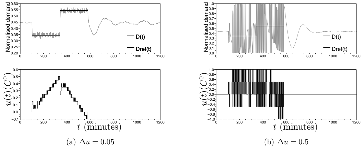
Figure 7: LM scenario on a population of 10000 ACs between t = 100 and t = 580 (minutes). The control aims to make the normalised power output D(t) follow the reference signal D_{\text{ref}}(t) (top plot). The control signal u(t) is shown in the bottom plots. The quantisation of u(t) is \Delta u = 0.05 for (a) and \Delta u = 0.5 for (b).
