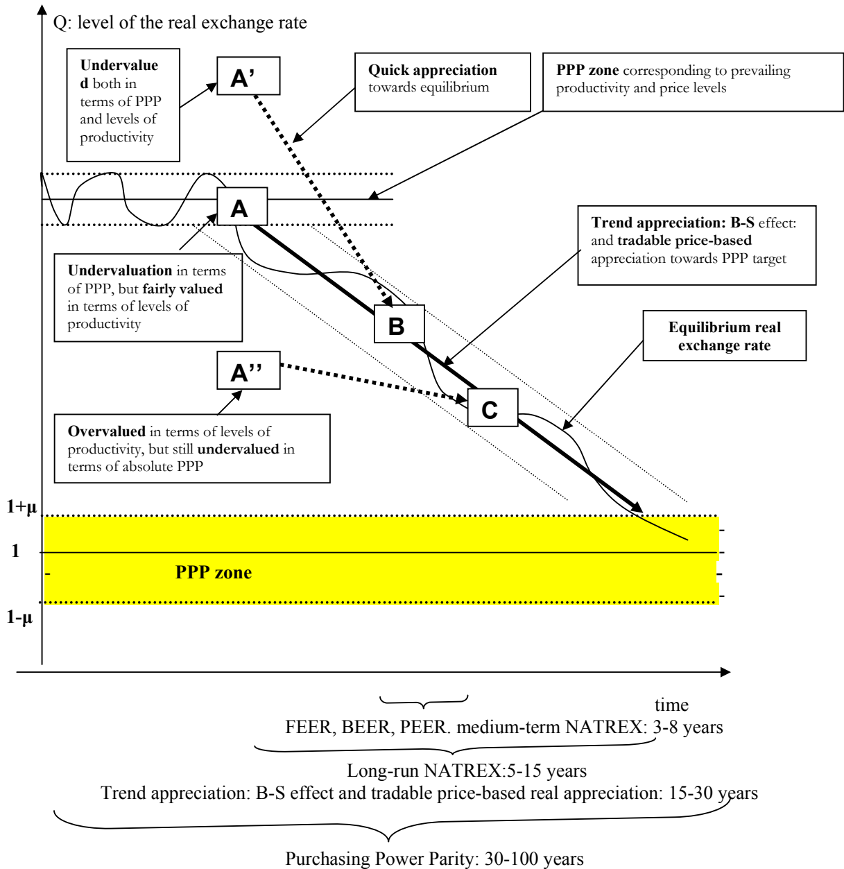
Figure 4. Trend Appreciation of the Equilibrium Real Exchange Rate
