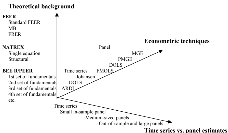
Figure 6. The three-dimensional space of equilibrium exchange rates
