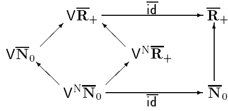
Figure 2: Two functions named \overline{id}
