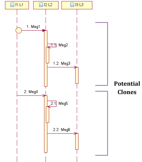
Fig. 2. Example of potential clones
