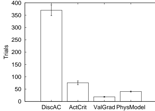
Figure 5: Comparison of learning speeds with discrete and continuous actor-critic and value-gradient based policies with an exact and learned physical models. The ordinate is the number of trials made until ten successful swing-ups.
