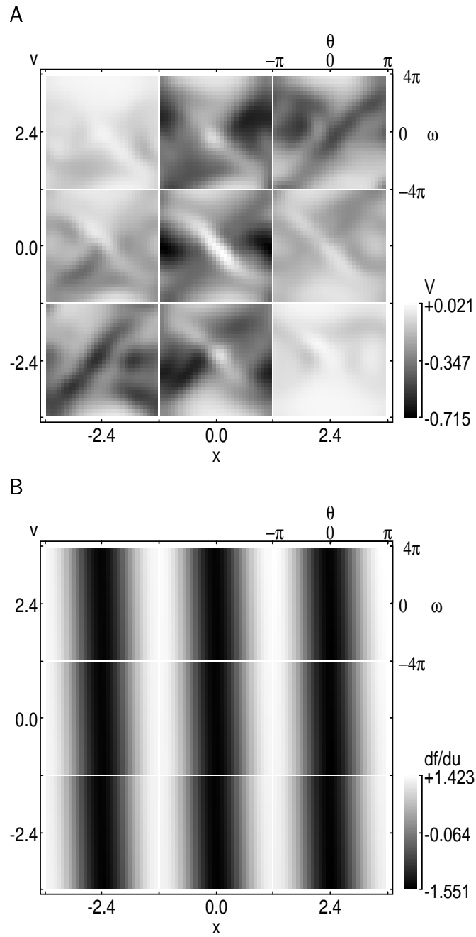
Figure 9: (A) The landscape of the value function for the cart-pole swing-up task. (B) The learned gain model \frac{\partial \dot{\omega}}{\partial u} .
