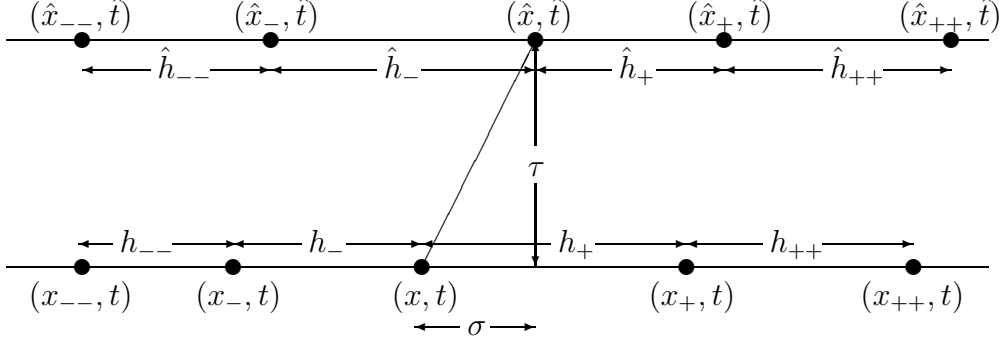
Figure 2: Lattice for the invariant discretization of the heat and Burgers equations (6 points) and the KdV equation (10 points).
