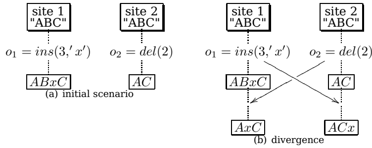
Figure 1: Divergence problem
