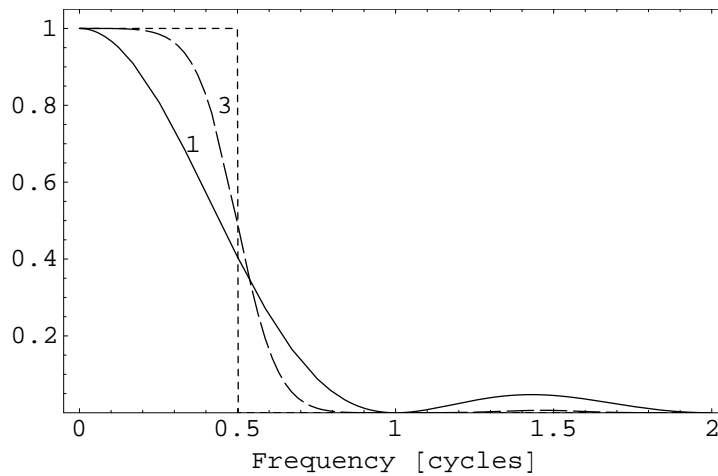
Fig. 5: Frequency response of the spline interpolators of degree n=1 and 3. As n increases, the spline interpolators tend to the ideal lowpass filter (dotted line).
