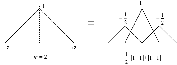
Fig. 9: Illustration of the two-scale relation for the linear B-spline.
