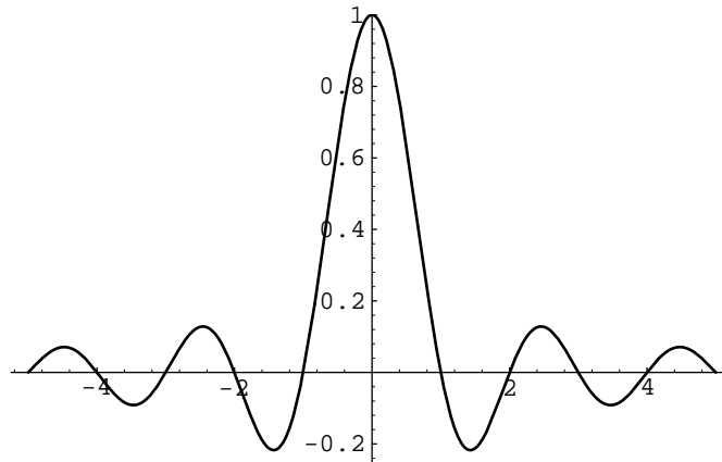
Fig. 4: Cardinal (or fundamental) cubic spline.
