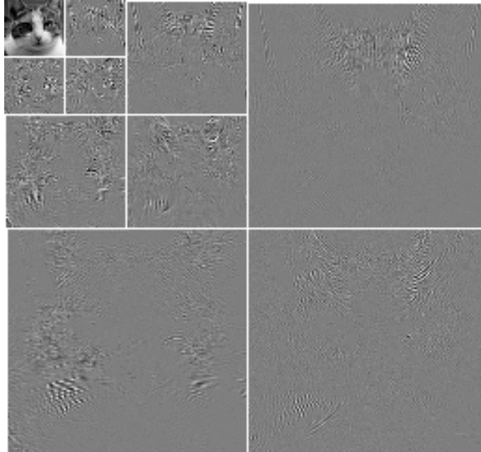
Fig. 11: Separable cubic spline wavelet transform corresponding to the multiresolution decomposition in Fig. 10.
