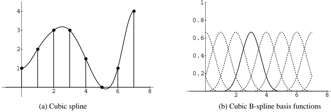
Fig. 2: Example of a cubic spline signal that is represented as a linear combination of shifted cubic B-splines.
