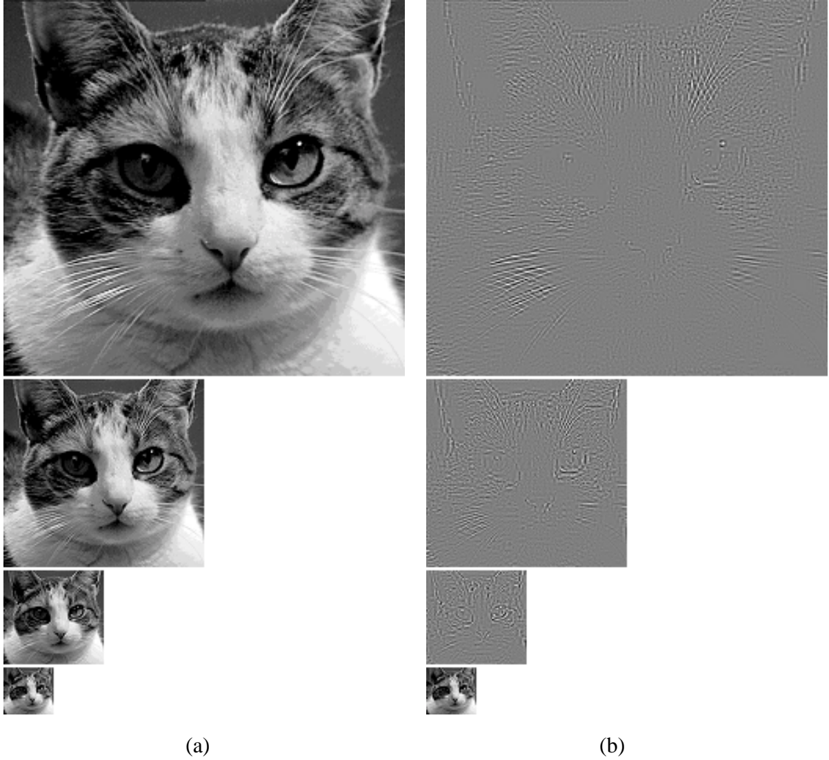
Fig. 10: Cubic spline multiresolution image approximation. (a) Cubic spline pyramid \{P_0s, P_2s, P_4s, P_8s\} . (b) Corresponding error pyramid: \{P_0s - P_2s, P_2s - P_4s, (P_4s - P_8s), P_8s\} . What is displayed are the samples of those splines at the location of the knots (cardinal representation).
