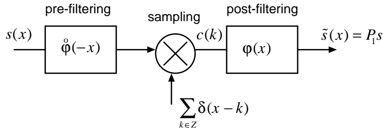
Fig. 6: Least-squares spline approximation. The analog input signal s(x) is prefiltered with \overset{\circ}{\phi}(-x) and sampled thereafter to yield the generalized spline coefficients c(k) = \langle s(x), \overset{\circ}{\phi}(x - k) \rangle . The sampling is modeled by a multiplication with a sequence of Dirac deltas. The spline approximation \tilde{s}(x) = \sum_{k \in \mathbb{Z}} c(k) \phi(x - k) is then obtained by post-filtering with \phi(x) .
