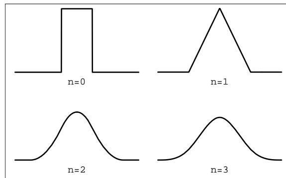
Fig. 1: The centered B-splines of degree 0 to 3.
