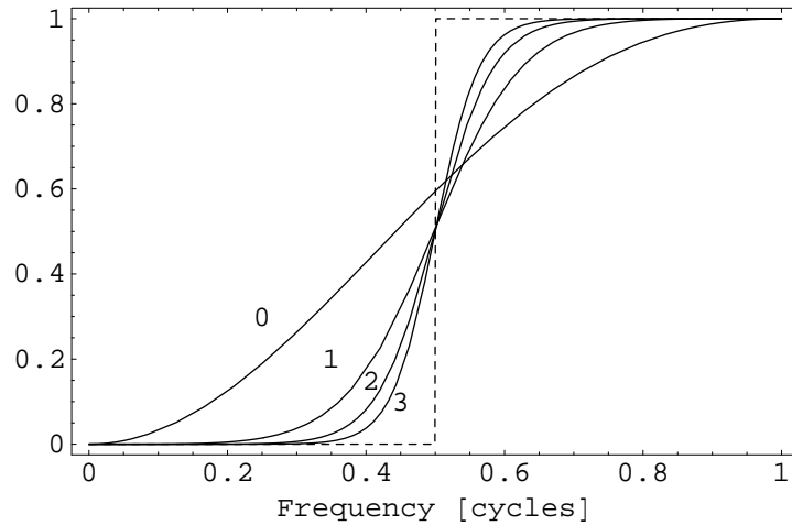
Fig. 8: Frequency plot of the error kernels for the least-squares spline approximations of degree n=0,1,2,3 . Below the Nyquist frequency \omega = \pi , the kernels (and therefore the errors) tend to be smaller for splines of higher degree.
