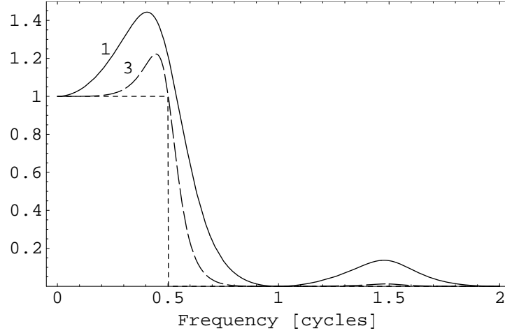
Fig. 7: Frequency response of the optimal spline prefilters of degree n=1 and 3. As n increases, the optimal spline prefilters tend to the ideal lowpass filter (dotted line).
