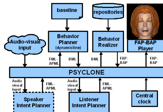
Figure 1. Greta architecture.
