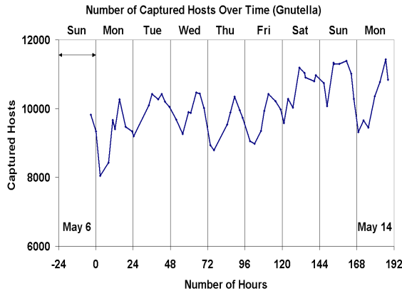
Figure 2: Number of Gnutella hosts captured by our crawler over time
