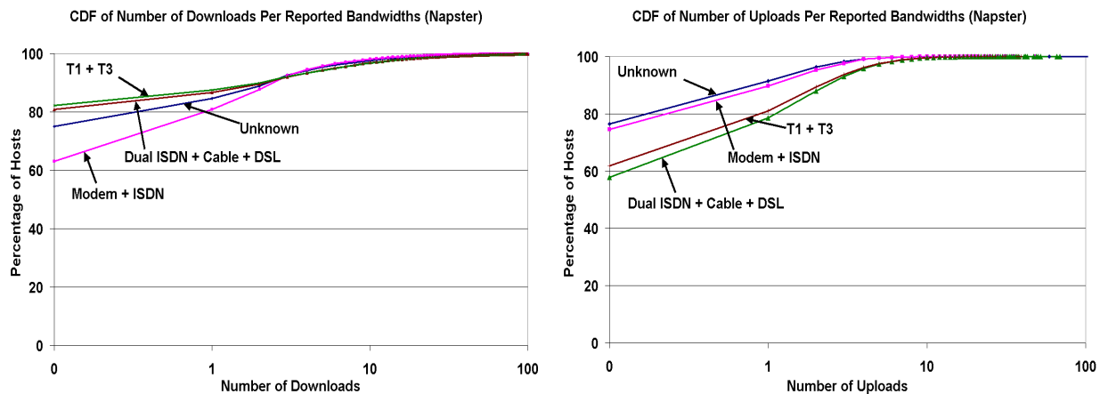
Figure 8. Left: The number of downloads by Napster users, grouped by their reported bandwidths; Right: The number of uploads by Napster users, grouped by their reported bandwidths.
