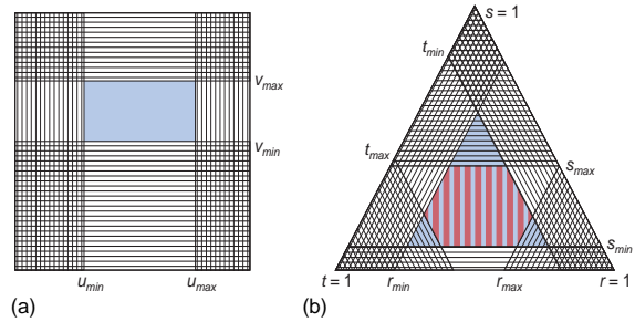
Figure 4: Bézier Clipping in the parametric domain (candidate region highlighted in blue): (a) Rectangular (tensor product) domain (b) Triangular (barycentric) domain
