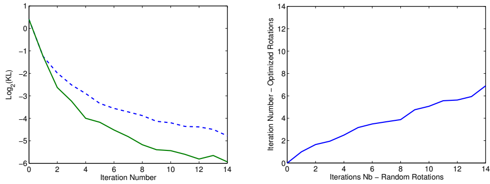
Fig. A.4. Optimised rotation sequence speed up for N = 2 . On the left, the averaged evolution of the log Kullback Leibler divergence for 100 simulation for both a random sequence of rotations and an optimised sequence of rotations. On the right, the correspondence between iteration numbers for both strategies. It requires in average 53% less iterations for N = 2 when using an optimized rotation sequence.
