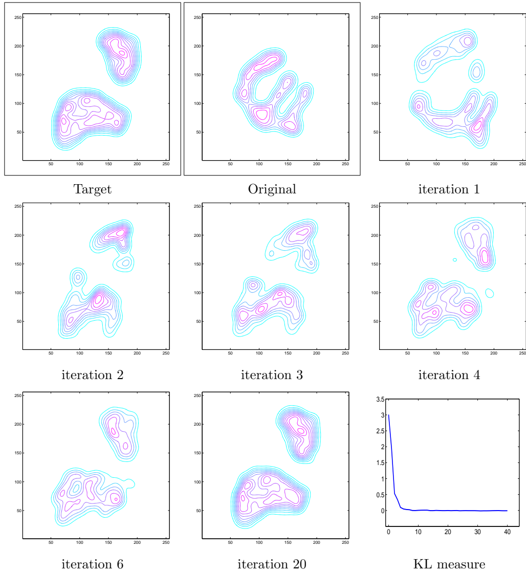
Fig. A.1. Example of a two dimensional pdf transfer using IDT . The decrease of the Kullback-Leibler divergence illustrates the convergence of method.
