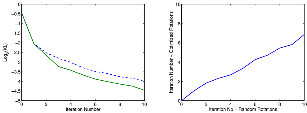
Fig. A.5. Optimised rotation sequence speed up for N = 3 . On the left, the averaged evolution of the log Kullback Leibler divergence for 100 simulation for both a random sequence of rotations and an optimised sequence of rotations. On the right, the correspondence between iteration numbers for both strategies. It requires in average 33% less iterations for N = 3 when using an optimized rotation sequence.
