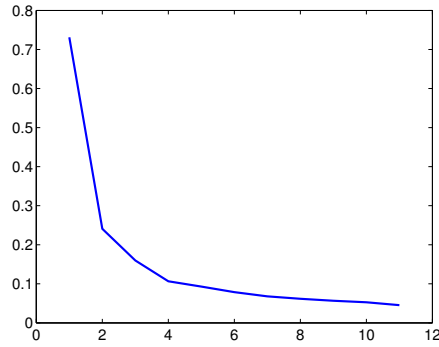
average KL divergence, in 3D
