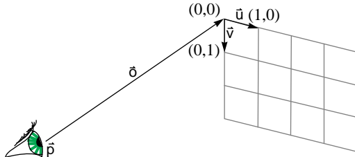
FIGURE 3. The center-of-projection, \bar{p} , a vector to the origin, \bar{o} , and two spanning vectors ( \bar{u} and \bar{v} ) uniquely determine the planar projection.
