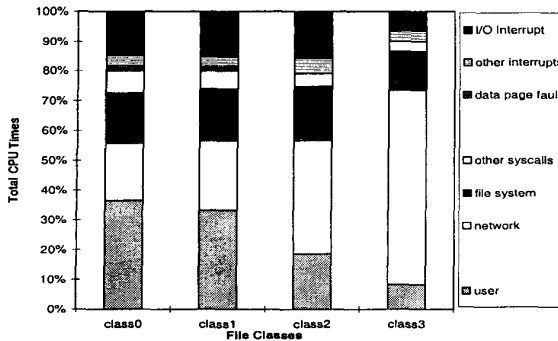
Figure 2: Apache CPU Time for different file sizes
