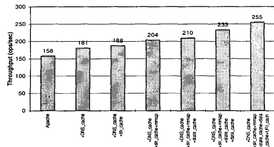
Figure 3: SPECweb96 Results of the Enhanced Apache
