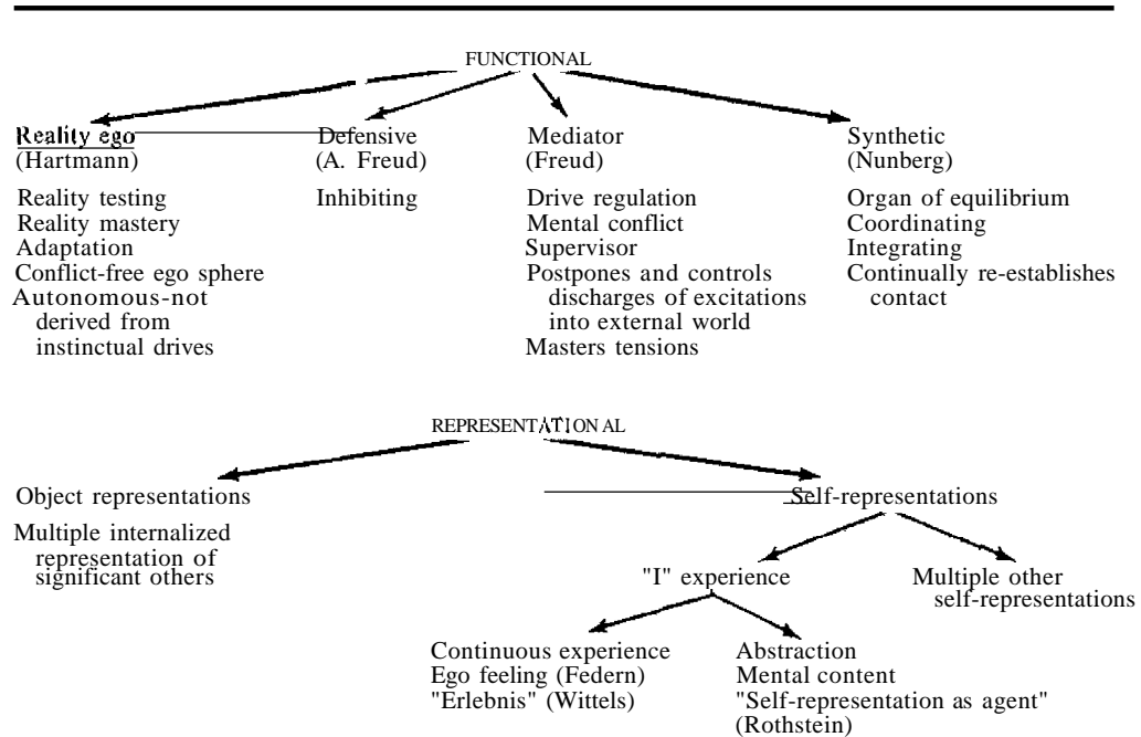
FIGURE I SYSTEM EGO
