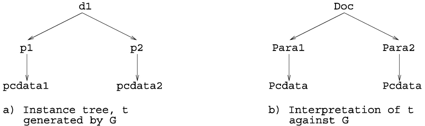
Figure 1 An instance tree generated by G_1 , and its interpretation against G_1 . We use unique labels to represent the nodes in the instance tree.
