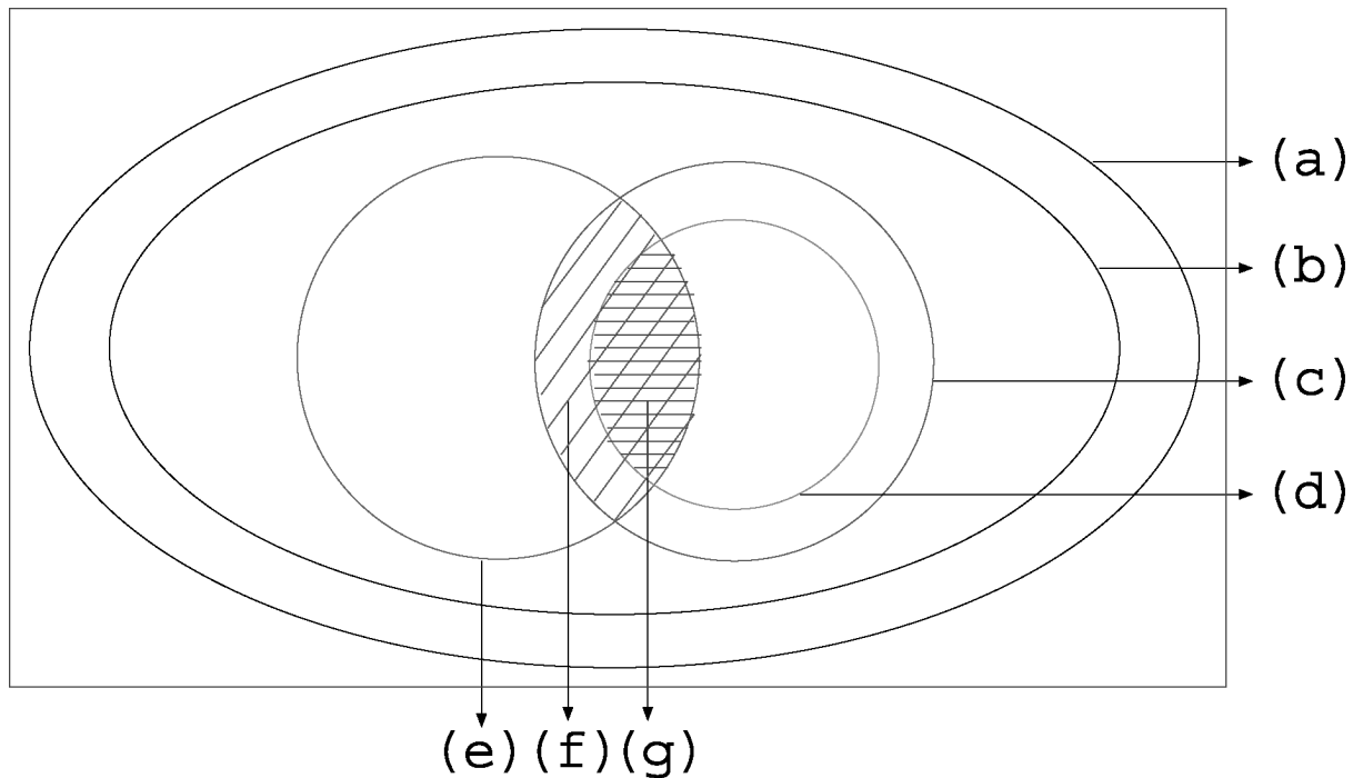
Figure 2 The expressive power of the different regular tree grammars: (a) regular tree grammars (RELAX Core, XDuce, TREX), (b) restrained-competition tree grammars (c) single-type tree grammars (XML-Schema) (d) local tree grammars (DTD)
