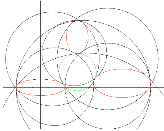
Fig. 5. All eight solution circles (black and green) tangent to three given ellipses (red).
