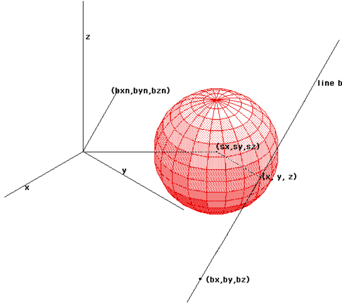
Fig. 7. Parameterization of line tangent to sphere in three-space.
