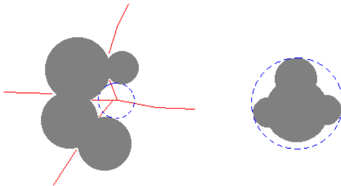
Fig. 3. Left: Medial axis (lines) for a very simple 2D molecule (gray atoms) with one medial disc shown (dashed circle). Right: The diameter of the enclosing (dashed) circle around this molecule quickly confirms that it is too big to fit into the pocket in the molecule on the left.
