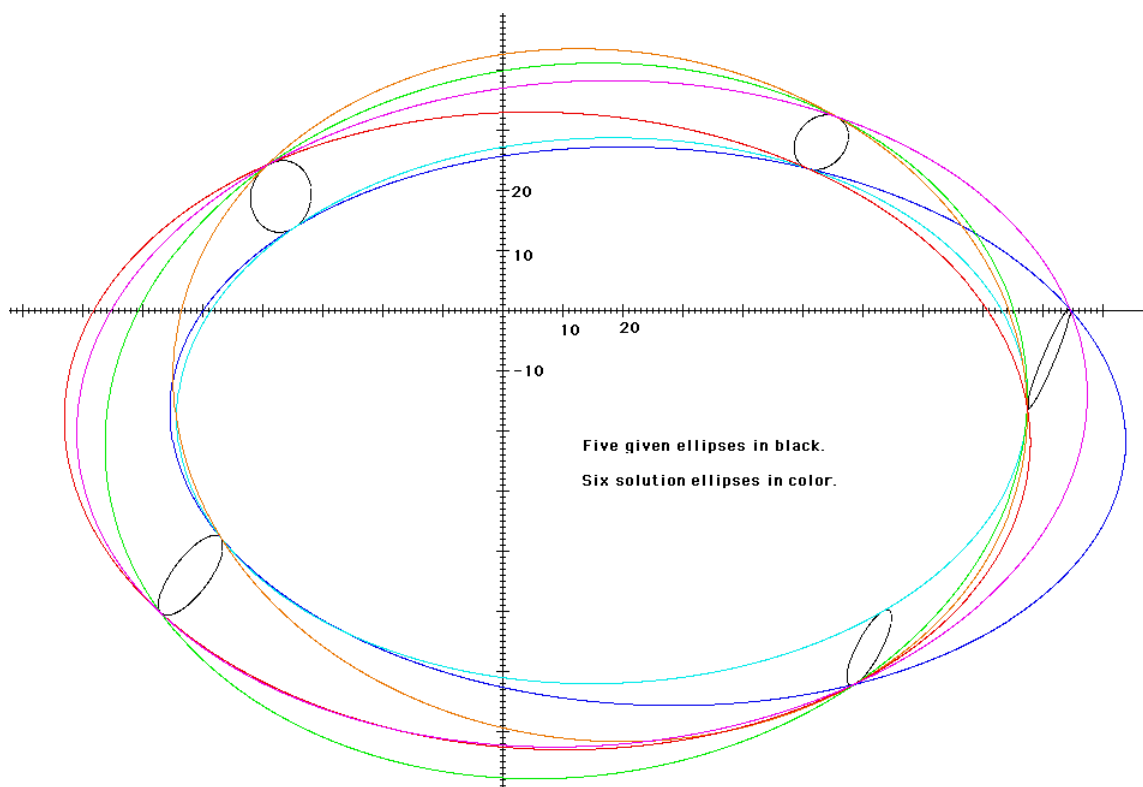
Fig. 8. Six solution conics tangent to five given ellipses.
