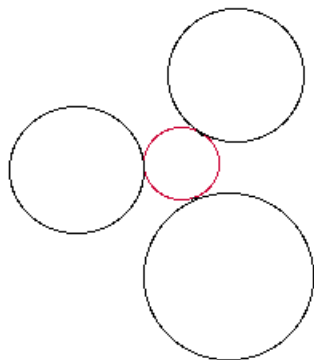
Fig. 1. Special case, two dimensions, where all circles are mutually tangent, solution circle in red.
