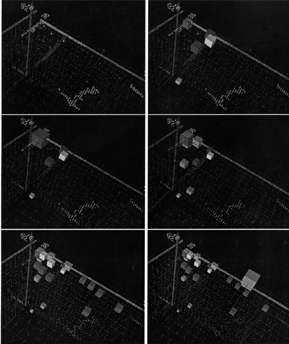
Figure 8. The shuttle dataset projected on the three most discriminatory axes. Color/shading denotes the class of instances and the cube sizes correspond to the instance weights. Each picture shows one AdaBoost trial, where progression is from the top left to top right, then middle left, etc. A color version of this figure can be found in http://robotics.stanford.edu/~ronnyk/vote Boost Graph.ps.gz .
