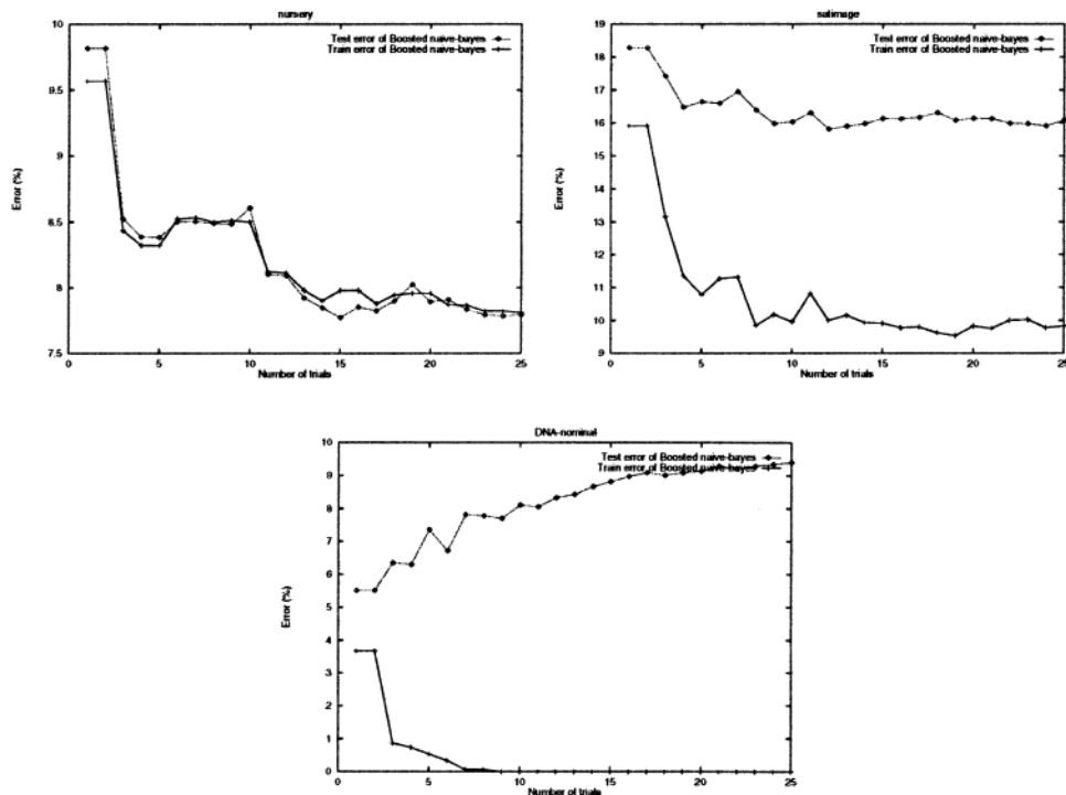
Figure 12. Trial graphs for selected datasets showing different behaviors of Naive-Bayes and AdaBoost. The graphs show the test set and training set errors as the number of trials increases. Each point is an average of three runs, each of which is based on 25 trials/replicates. Nursery represents the classical theoretical scenario where the test set error tracks the training set error because Naive-Bayes is a simple classifier; this case was fairly rare. Satimage is an example where the training set error and test set errors decrease and asymptote. DNA represents a most interesting example, where the training set error went down to zero as the theory predicts, but the test set error increased . Note that the y-axis ranges vary.
