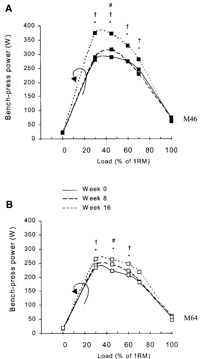
Fig. 4. Average power-load curve in the bench-press action in M46 (A) and M64 (B) at weeks 0, 8, and 16 during the 16-wk strength-training period. Significant difference ( P < 0.05 ) between # weeks 0 and 8 , * weeks 0 and 16 , and † weeks 8 and 16 . Arrows denote time course of power gain.
