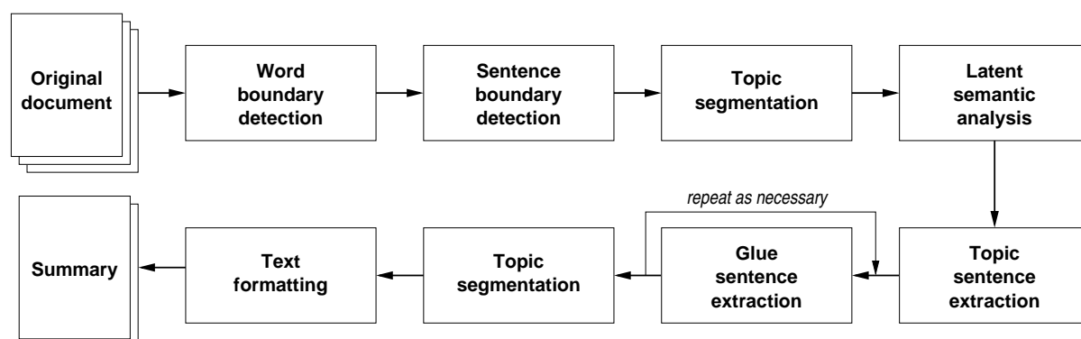
Figure 2.1: Summarizer architecture
