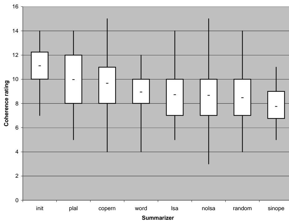
Figure 3.4: Summarizer coherence ratings
