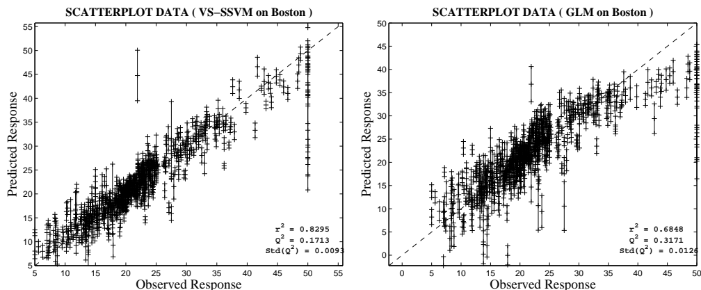
Figure 2: On Boston Housing data; left : VS-SSVM result; right : stepwise regression result.
