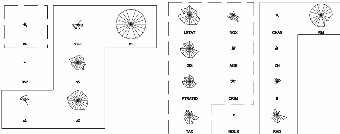
Figure 3: Starplots for left : the synthetic data and right : the Boston Housing data. Dotted and solid boxes contain non-positive and non-negative weighted variables.
