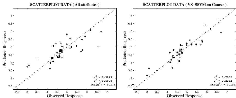
Figure 4: Left : Cancer full data; right : Cancer with variable selection.
