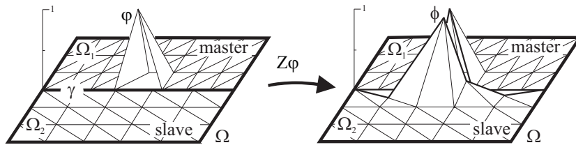
FIGURE 2.1. Construction of a basis function of \mathcal{V}_h
