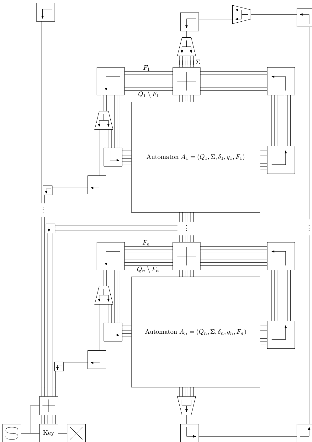
Fig. 4. Non-empty intersection simulation for several finite automata.
