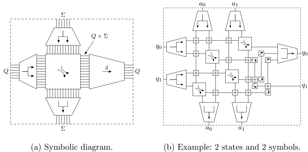
Fig. 3. Transition simulation of an automaton.
