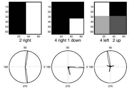
Fig. 5. Top: Different deviation of key-points from centers of masks. Bottom: Corresponding D_0(\theta) .
