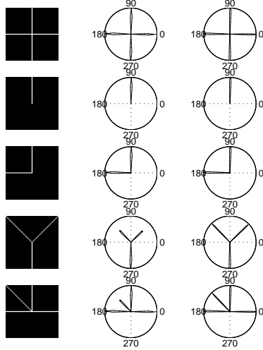
Fig. 3. Left: Synthetic line junction images with the size of 65 \times 65 pixels and line width of 1 pixel. Middle: Averaging outputs using the rectangle averaging filter defined in equation 4 with W = 6^\circ , R_{min} = 3 , R_{max} = 15 . The numbers around circles indicate angles in degree. Right: Corresponding Smoothing outputs P_0(\theta) using the Gaussian smoothing filter with same parameters. Both filters show good performances. But the normalization of the Gaussian filter is better (row 4 and 5).
