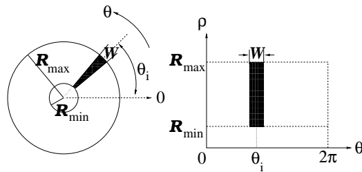
Fig. 1. Mask centered at angle \theta_i . Left: Original mask with keypoint at the center of the circle. Right: Mask with \theta and \rho as Cartesian coordinates, R_{max} and R_{min} are radial boundaries of the mask, W is the angular width of the mask.
