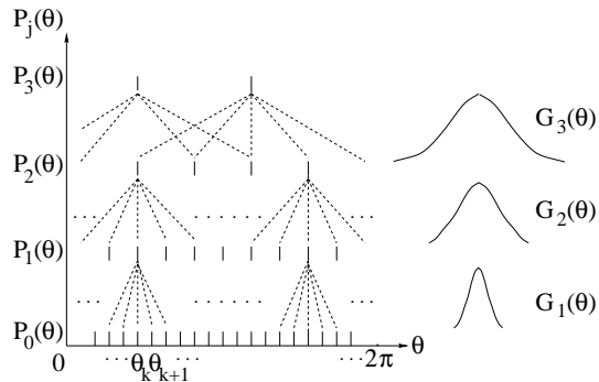
Fig. 2. Left: Polar pyramid structure, P_0(\theta) is the output of smoothing Gaussian filter. P_j(\theta)(j = 1, 2, \dots) are higher levels after sub-sampling with generating kernels S_2 or S_3 . Right: Corresponding interpolation functions at different levels. They are Gaussian functions with different scales.
