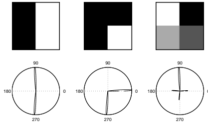
Fig. 4. Top: Synthetic edge junctions. Bottom: Polar plots of D_0(\theta) . The local maxima show the orientation of edges. R_{min} = 3 , R_{max} = 15 .
