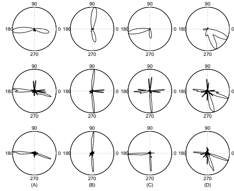
Fig. 6. Left: Parkbench with edge junctions. A : horizontal edge; B : vertical edge; C : corner; D : 'T' junction. Right Row 1: Steerable wedge filter results using 30 basis filters with 19-tap size. Right Row 2: Derivative Outputs using angular averaging filter. The averaging filter is sensitive to high frequency component. Right Row 3: Derivative Outputs using Gaussian smoothing filter. The result is better than using averaging filter. R_{min} = 3, R_{max} = 9 .
