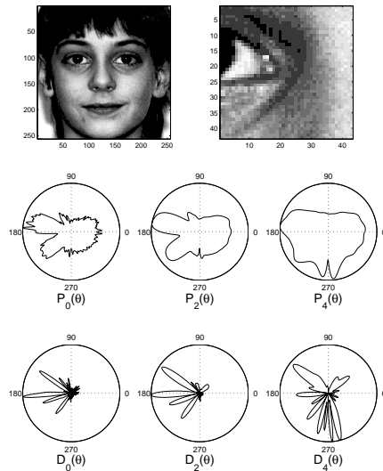
Fig. 8. Top left: Face of a child. Top right: Its left eye corner in detail. It can be regarded as combination of irregular wide lines and blurred edges disturbed by noise. Middle: orientational signals reconstructed from the first, third and fifth level of the polar pyramid. The eyelids are clear to see at the third level as two maxima at 135^\circ and 225^\circ . The local maximum near 180^\circ is due the white of the eye. Bottom: Corresponding D_j(\theta), j = 0, 2, 4 .
