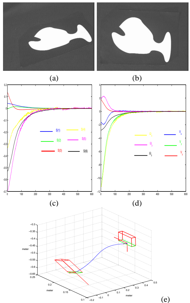
Fig. 3. Results for a complex motion: (a) initial image, (b) desired image, (c) visual features ( \mathbf{s} - \mathbf{s}^* ), (d) camera velocity \mathbf{T}_c , (e) camera 3D trajectory
