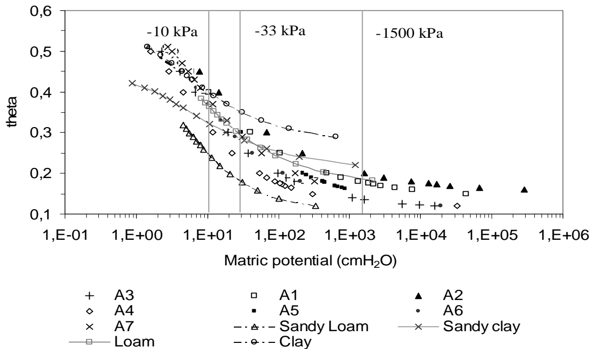
Figure 2. Water release curves for field sample soils and IGPB/T soil data set
