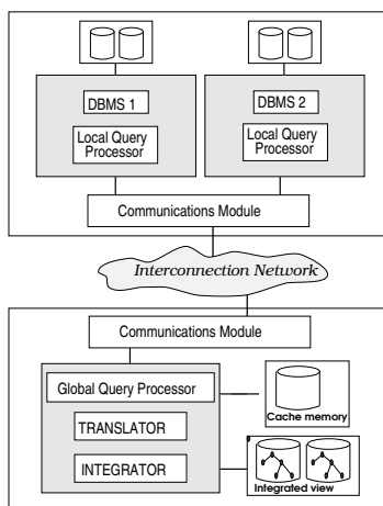
Figure 1: Architecture of the FDBS.
