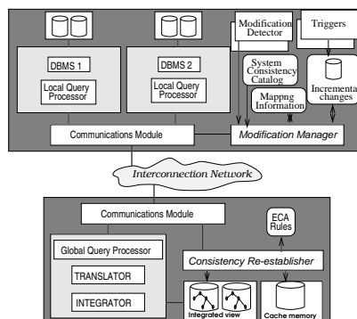
Figure 2: Architecture of the FDBS with the Monitor component.
