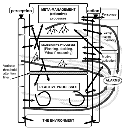
Figure 1: The CogAff Architecture
