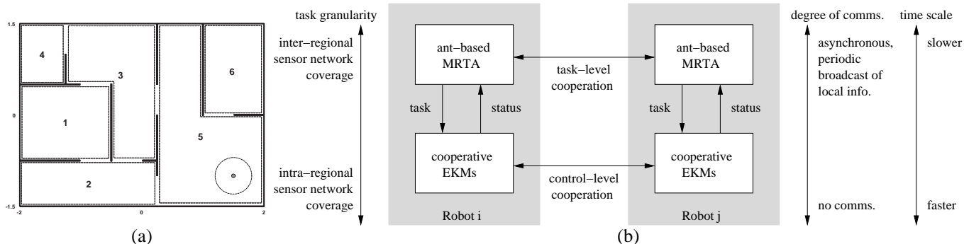
Figure 1: (a) A 4 m \times 3 m environment that is divided into 6 regions. The circle at the bottom right represents the robot’s sensing radius of 0.3 m (drawn to scale). The environment is 42.44 times as large as the robot’s sensing area. (b) Two-level integrated framework for multi-robot cooperation (MRTA = Multi-Robot Task Allocation, EKM = Extended Kohonen Map).
